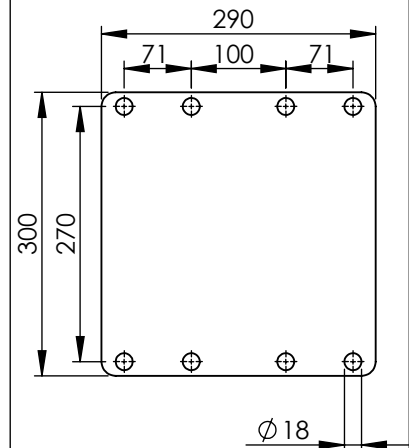
Gatenpatroon/hole pattern/ Bohrbild/motif de trous
